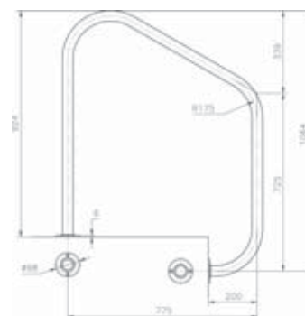
SPECIAL HANDRAIL
