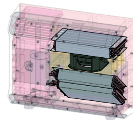
NEW INTERNAL ASSEMBLY
